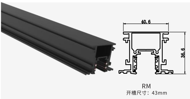
RM Size:40.6X36.6X48.8mm
