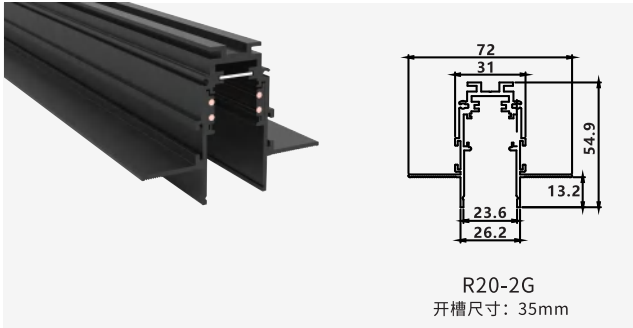
R20-2G Size:31X53X72mm
