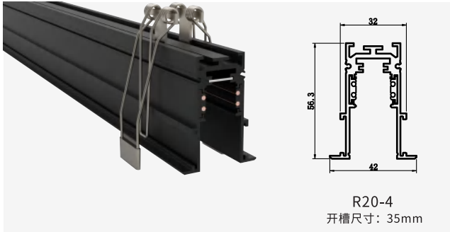
R20-4 Size:32X56.3X42mm
