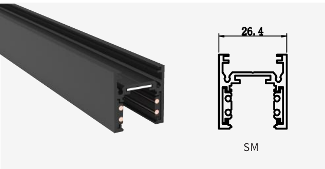
SM Size:26.4X26.4X26.4mm
