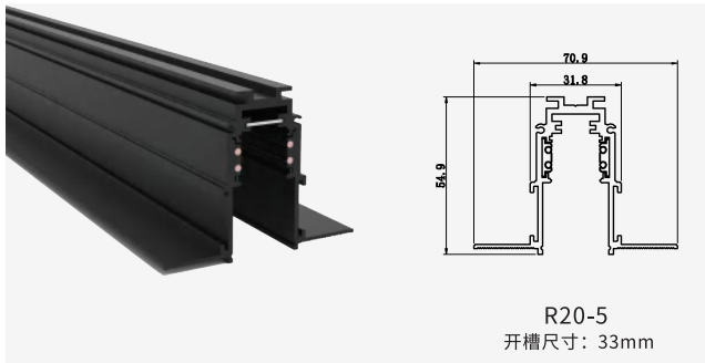
R20-5 Size:70.9X54.9X31.8mm
