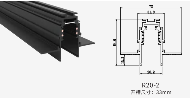
R20-2 Size:72X54.9X26.3mm
