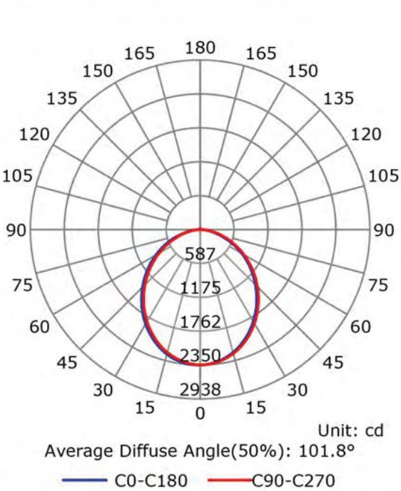
Luminous Intensity Distribution Curve
