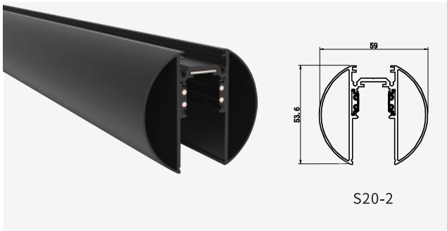
S20-2 Size:59X53.6X59mm
