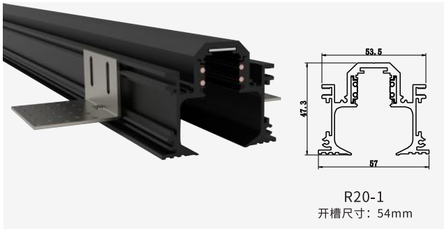
R20-1 Size:53.5X47.3X57mm
