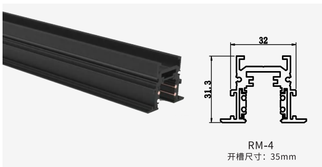
RM-4 Size:31.3X32X42mm
